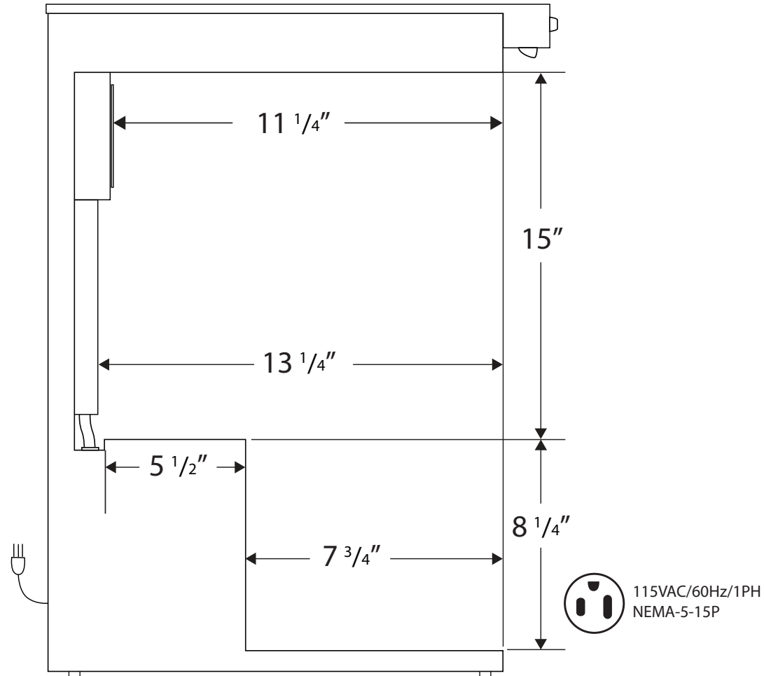
Side View
