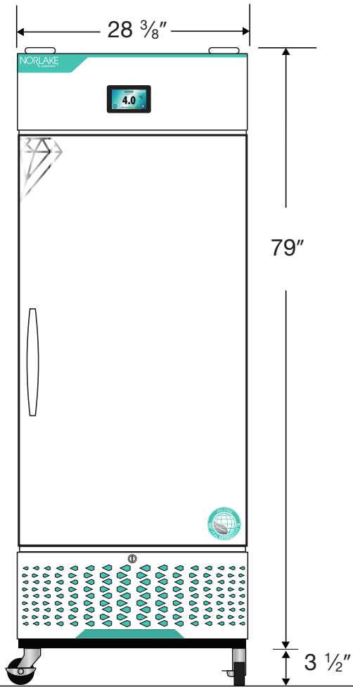
Front View
